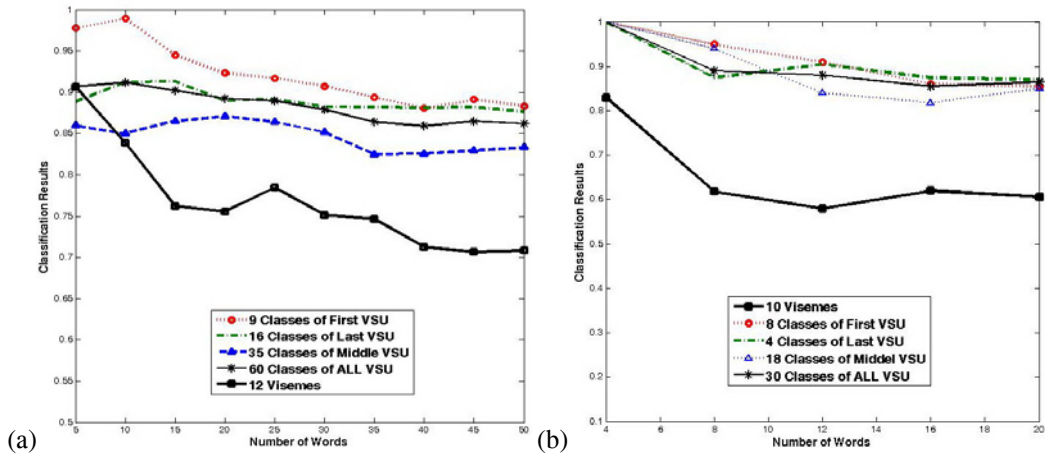
Fig. 12. Viseme vs. VSU Classification. (a) Speaker One. (b) Speaker two.
