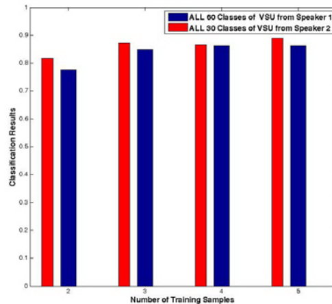
Fig. 13. Visual Speech Unit Classification with respect to the number (2-5) of training examples.
