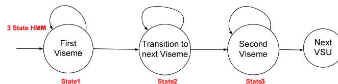
Fig. 11. HMM topology for VSU
