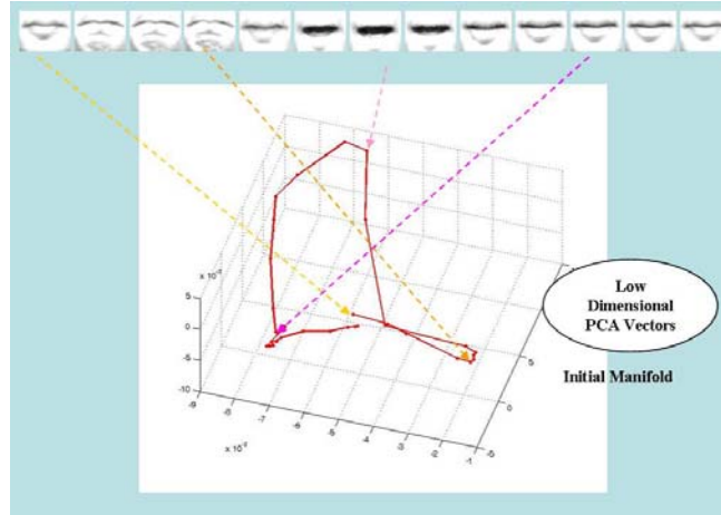
Fig. 2. EM-PCA manifold representation of the word “Bart”. Each feature point of the manifold is obtained by projecting the image data onto the low-dimensional EM-PCA space.
