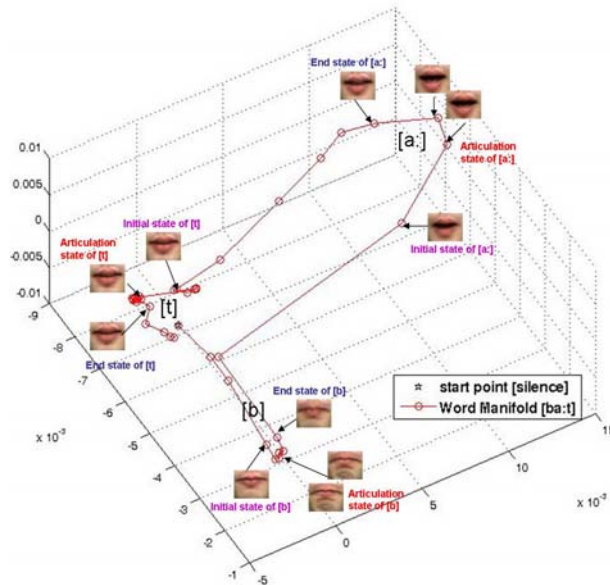
Fig. 4. EM-PCA points generated by images from the video sequence describing the word [ba:t].
