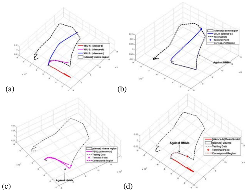
Fig. 10. VSU Registration and Classification. (a) The registration of three classes of the VSU Class 1: [silence-b] (red line); Class 2: [silence-ch] (purple line); Class 3: [silence-a:] (blue line) to the word manifold (black dotted line). (b) Registration between the [silence-a:] VSU mean model and the word manifold. (c) Registration between the [silence-ch] VSU mean model and the word manifold. (d) Registration between the [silence-b] VSU mean model and the word manifold. The [silence-ch] VSU mean model achieved the best matching cost (evaluated using a three-state HMM classification).
