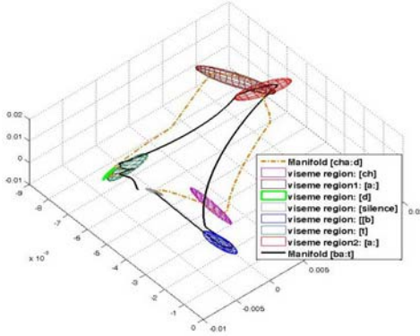
Fig. 6. Viseme feature space constructed for two different words. Word “Bart”-viseme [b], [a:] and [t]. Word “chard” – visemes [ch], [a:] and [d].
