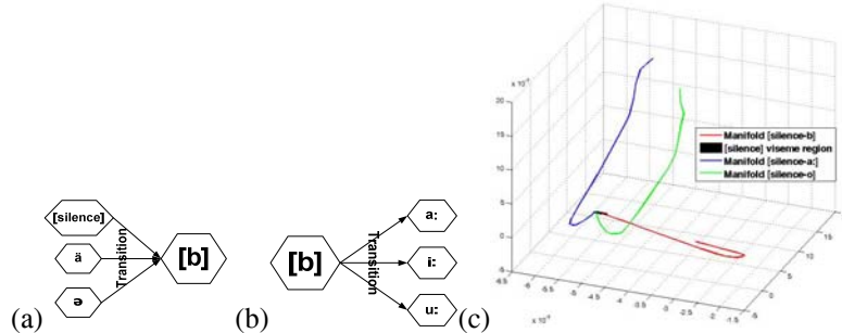
Fig. 7. Visual Speech Unit Examples. (a) VSU Prototypes: [silence-b], [ä-b] and [ə-b]. (b) VSU Prototypes: [b-a:], [b-i] and [b-u:]. (c) VSU Manifold for [silence] to visemes [b], [a:] and [o].
